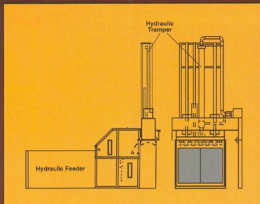
COMBINATION OF HYDRAULIC TRAMER & HYDRAULIC PUSHER FEEDER FOR "NDBDP" PRESS
