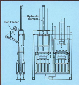
"NDBDP" PRESS WITH COMBINATION HYDRAULIC TRAMPER & MECH. BELT FEEDER
