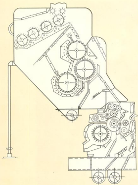
Sectional View showing Feeder and Gin internals
